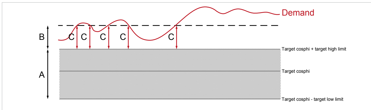
Fig. 3-26 RAPIDUS Mode Compensation Steps
