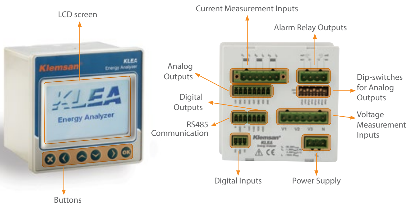
KLEA 324P Energy Analyzer
