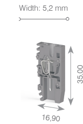
SC-PT 2.5
