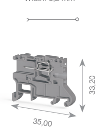
SC-PTR 2.5
