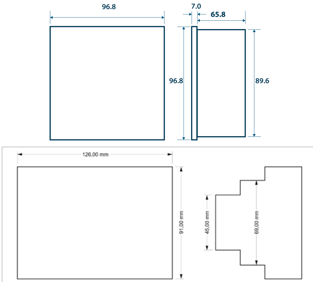
Figure 2-3 Dimensions for Klea 220P and POWYS 3121-3122
